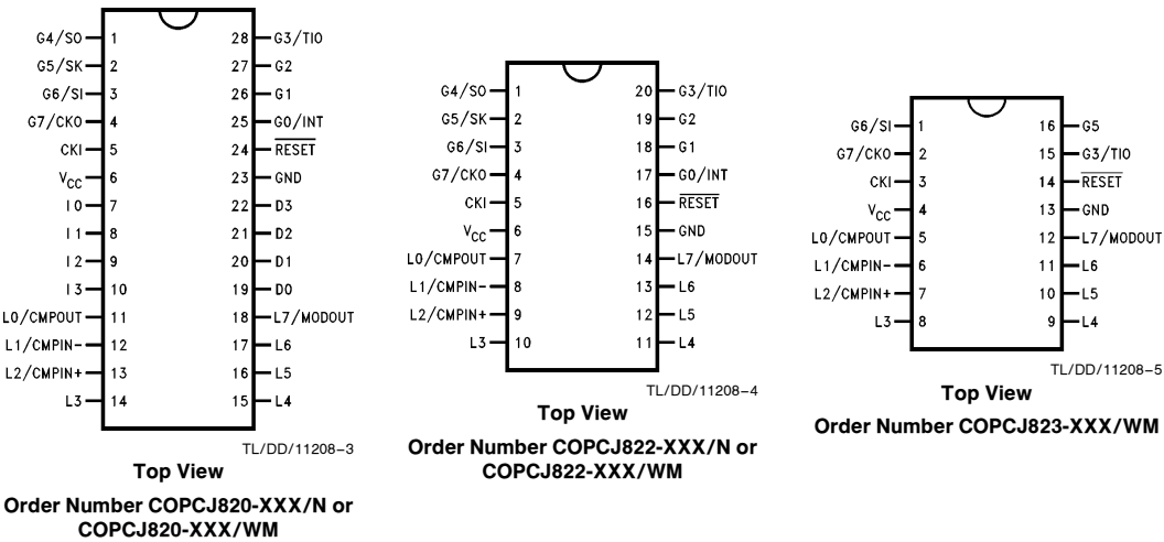
FIGURE 3. Connection Diagrams
